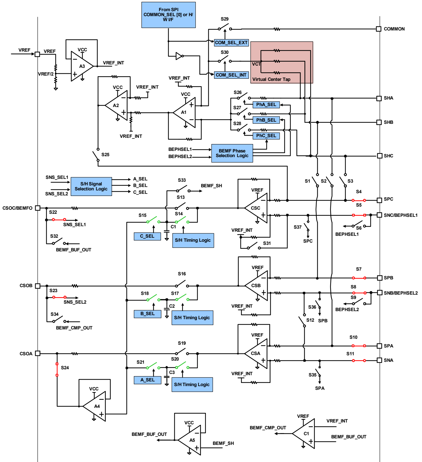
Figure 32. Configuration 5
