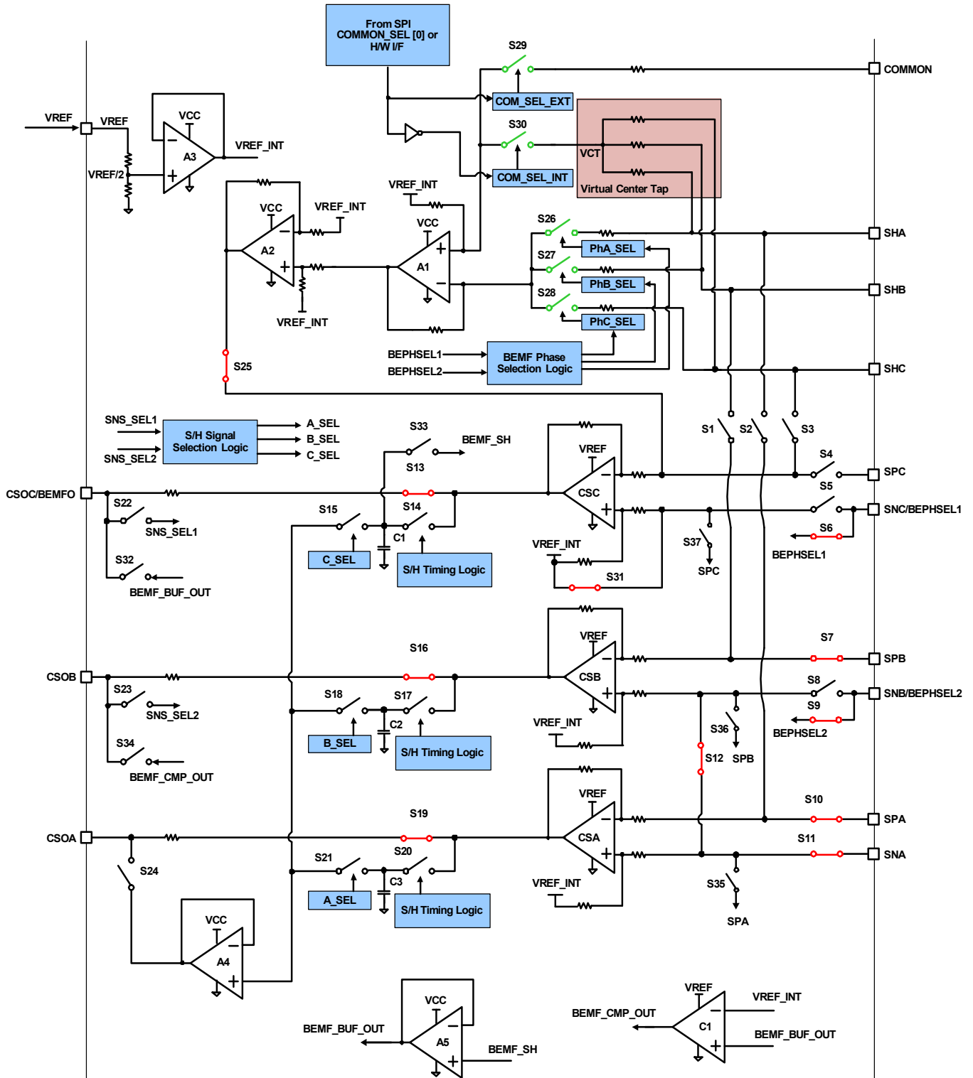
Figure 31. Configuration 4
