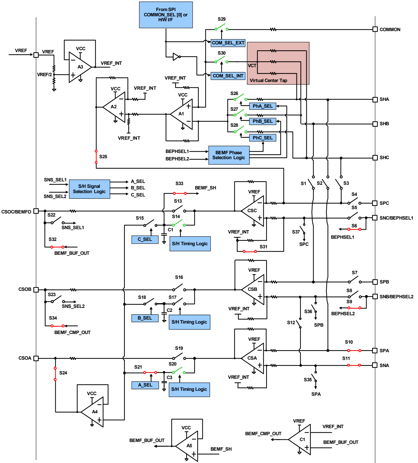
Figure 36. Configuration 9
