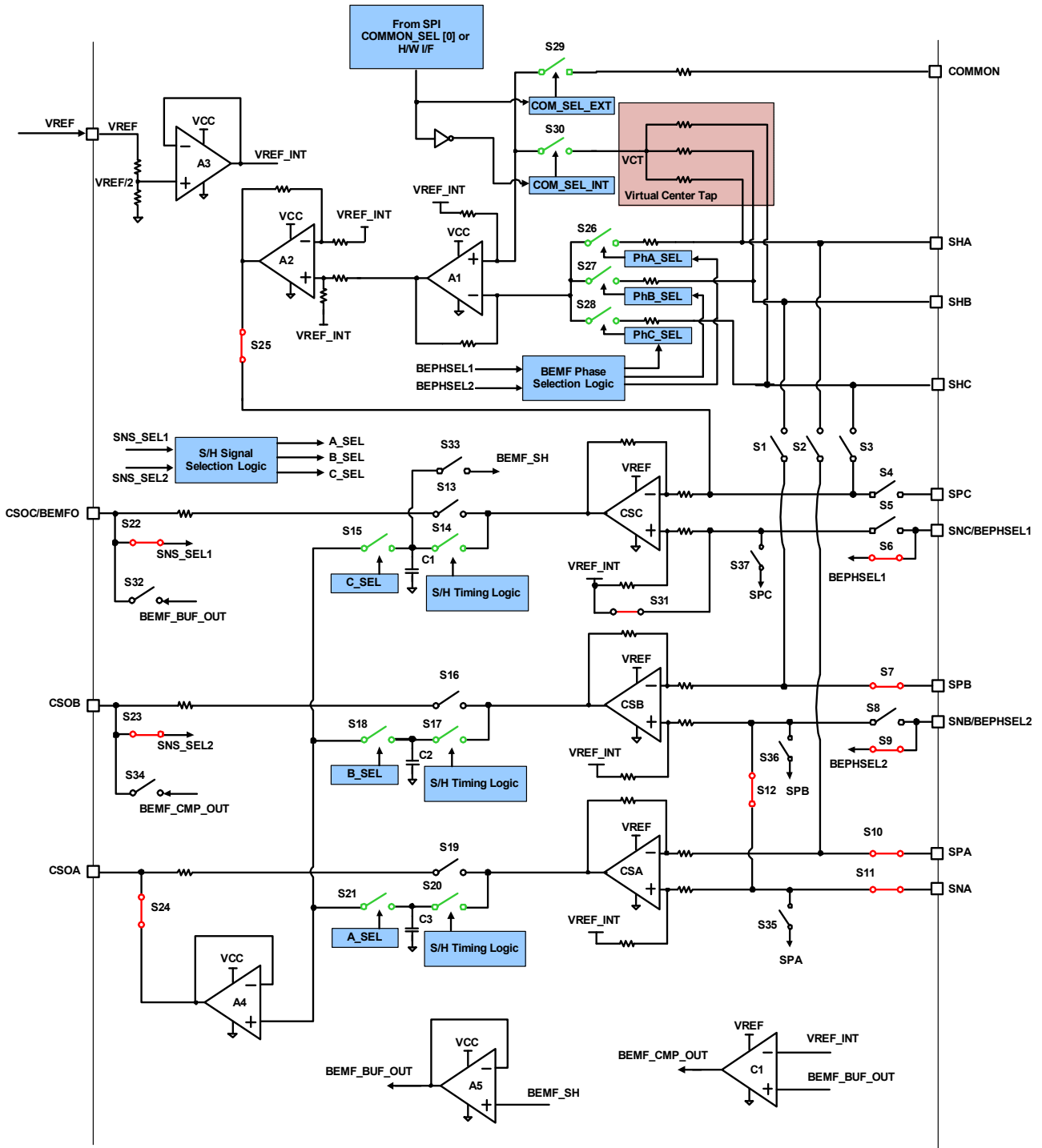
Figure 28. Configuration 1
