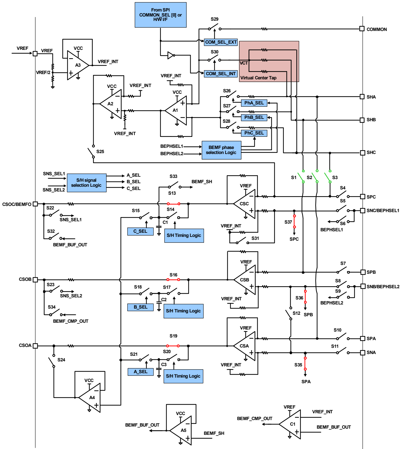
Figure 34. Configuration 7
