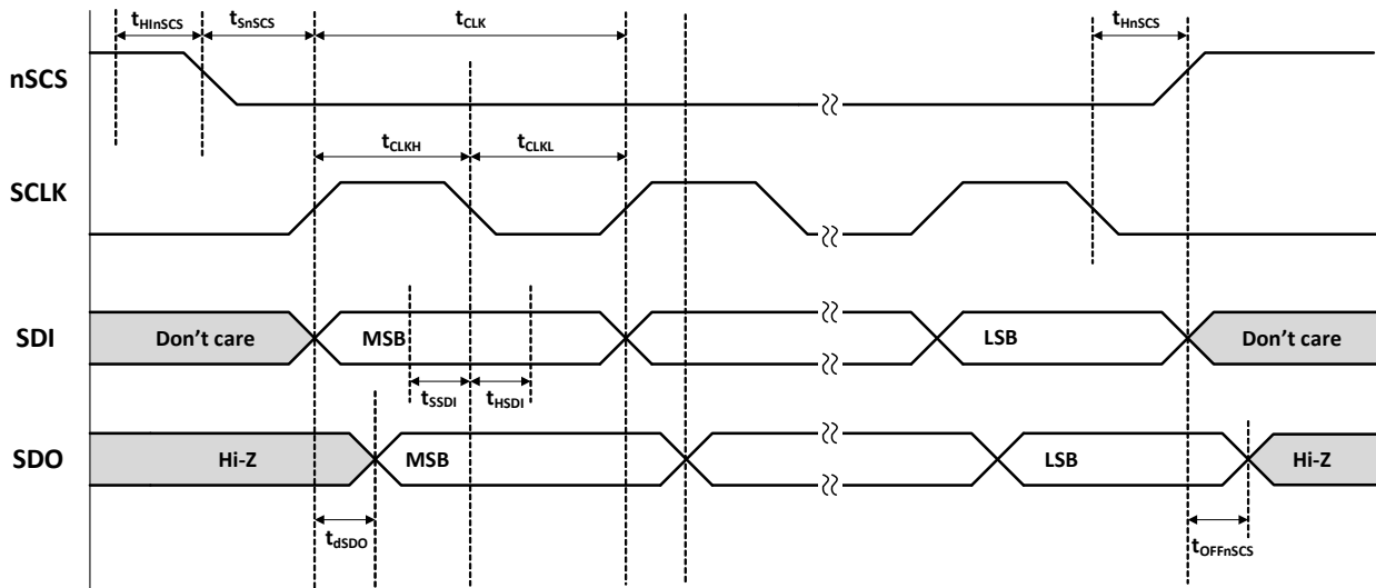
Figure 42. Timing Diagram
