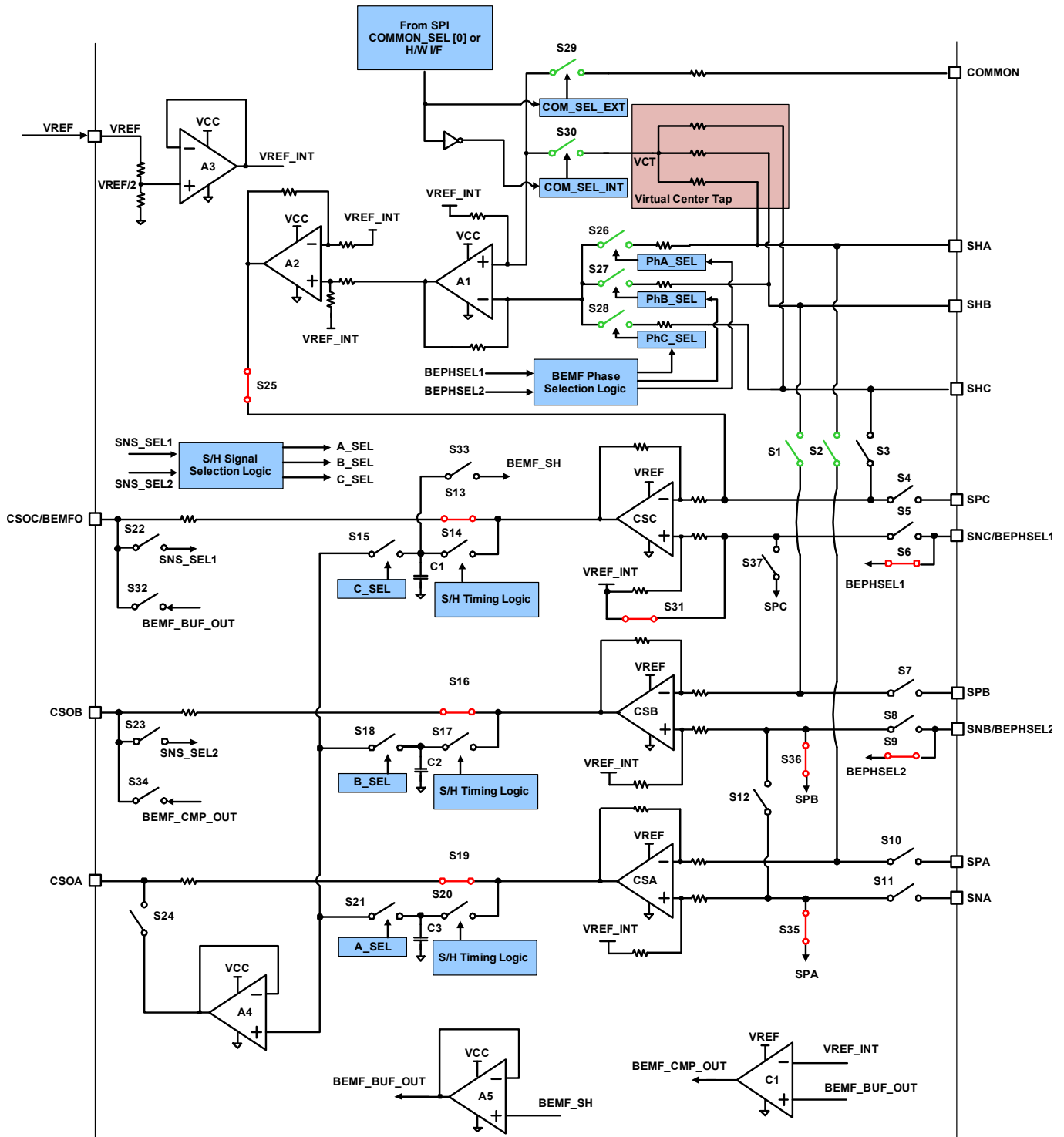
Figure 35. Configuration 8
