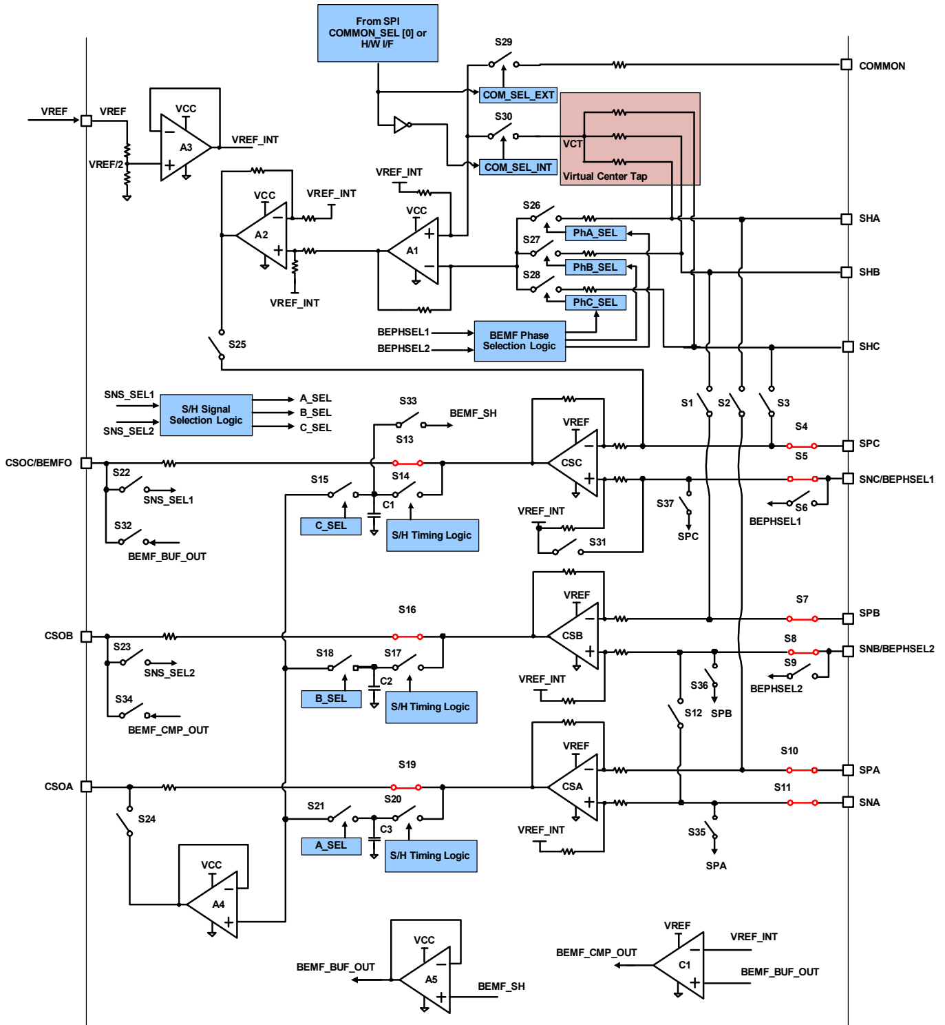
Figure 33. Configuration 6
