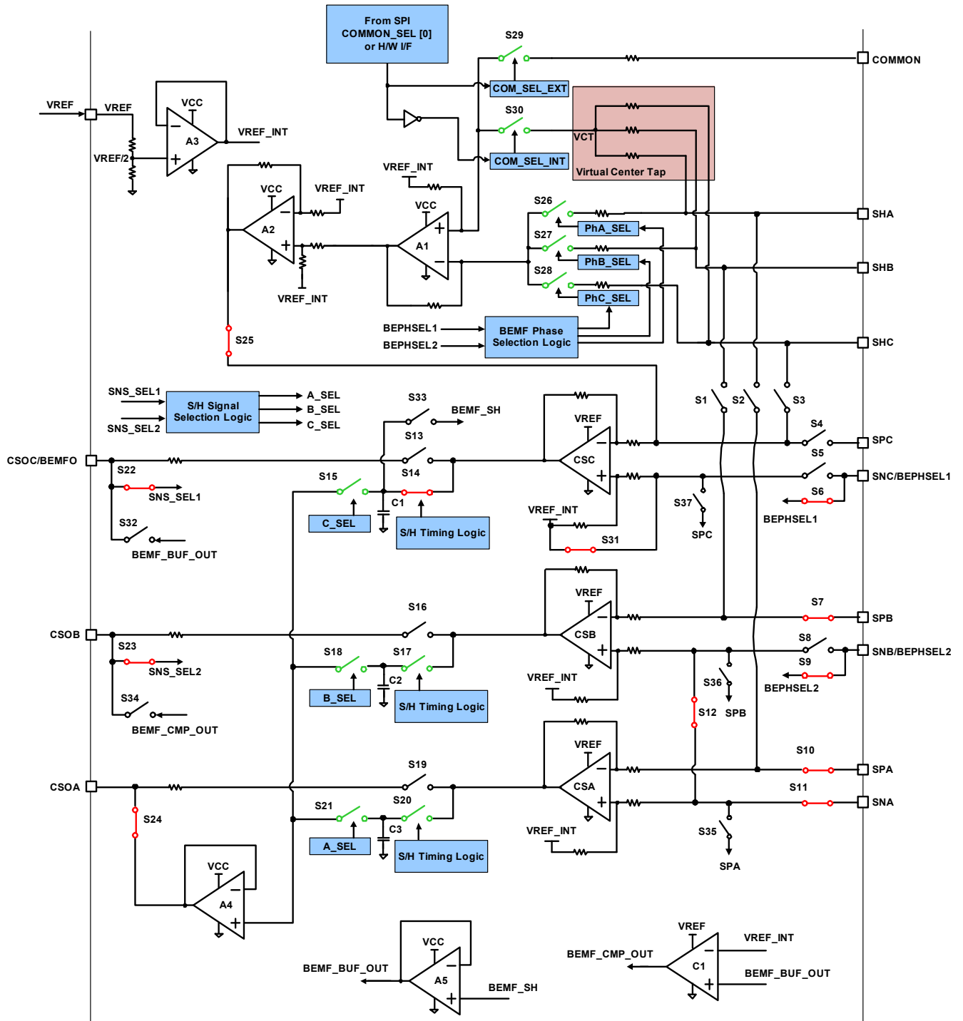
Figure 29. Configuration 2
