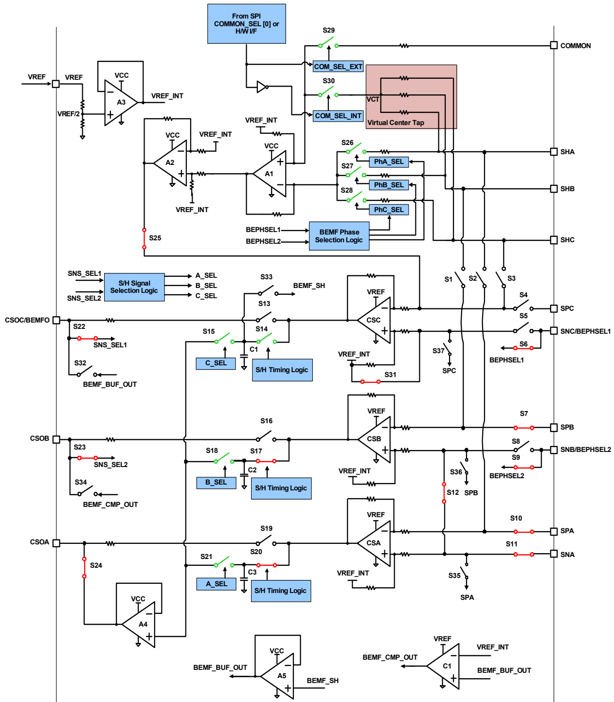
Figure 30. Configuration 3
