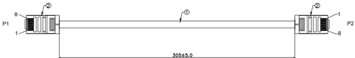
Cat6, RJ45 Plug to RJ45 Plug L=305mm
