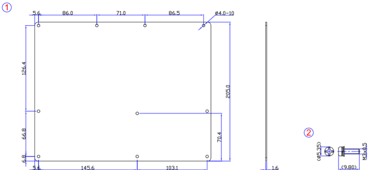
Adaptor Board for Formosa Enclosure
