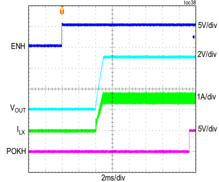
HV BUCK STARTUP THROUGH ENABLE ( V_{IN} = 24V , V_{OUT} = 5V , MODE = PWM, LOAD = 1.5A)
