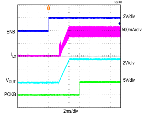
LV BUCK STARTUP THROUGH ENABLE ( V_{IN} = 5V , V_{OUT} = 1.8V , MODE = PWM, LOAD = 1.0A)
