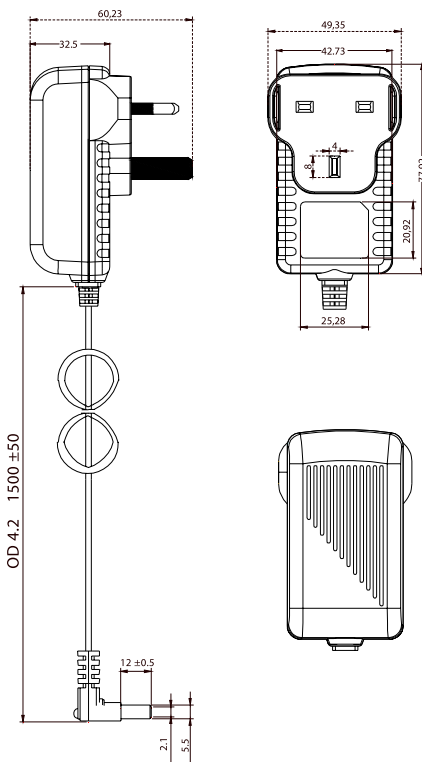
Dimensions : Millimetres Tolerance: ±0.2mm
