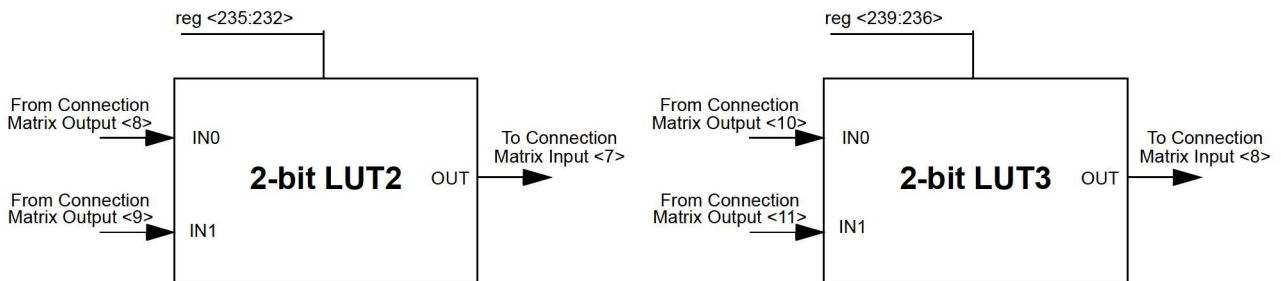
Figure 7. 2-bit LUTs
