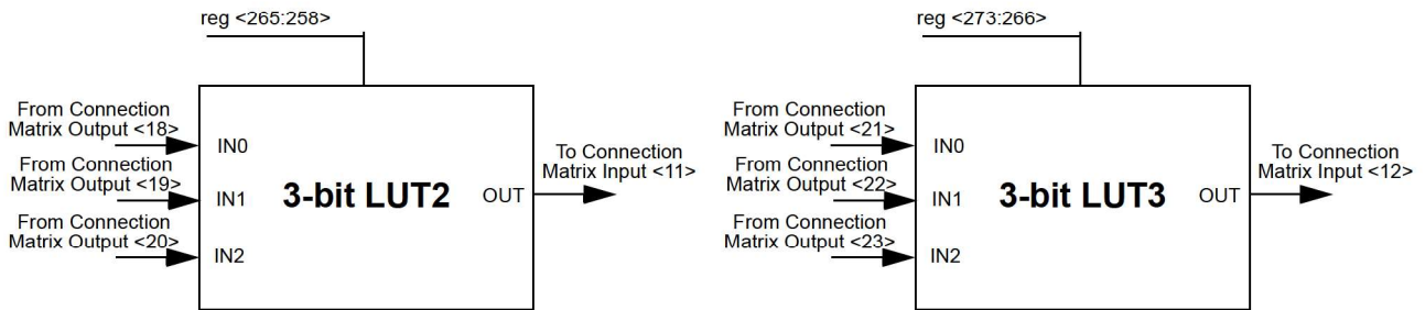
Figure 8. 3-bit LUTs
