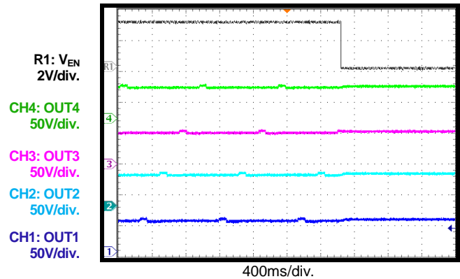
Shutdown through EN No PD connection
