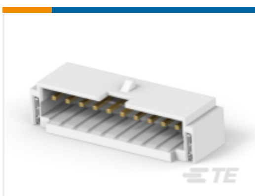
TE Part # 3-2381626-0 1.5P 10POS WTB R/A BRD W LATCH AU NAT
