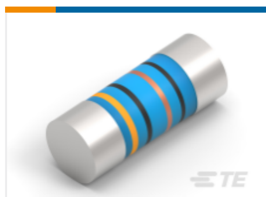
TE Part #3-2176315-5 MELF SMA_A 68K 0.1% 15PPM 0204 0.4W
