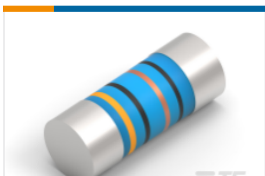
TE Part #1-2176315-5 MELF SMA_A 1K5 0.1% 15PPM 0204 0.4W
