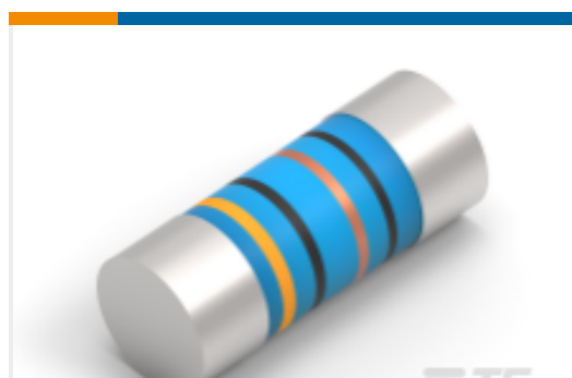
TE Part #2-2176315-6 MELF SMA_A 12K 0.1% 15PPM 0204 0.4W
