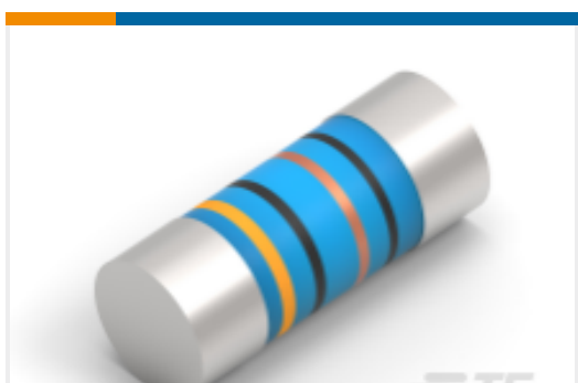
TE Part #3-2176315-1 MELF SMA_A 33K 0.1% 15PPM 0204 0.4W
