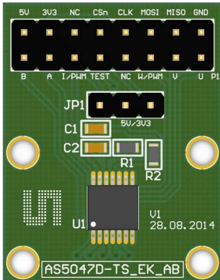
Adapter Board for AS5047D
