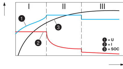
Figure 21 Charging characteristic
