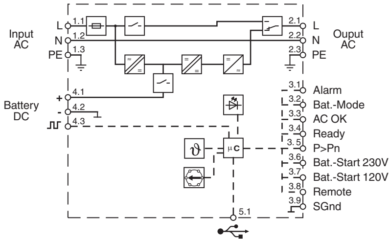
Figure 3 Block diagram
