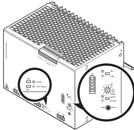
Figure 22 LED indicators
