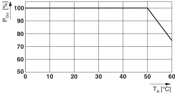
Figure 26 Temperature-dependent derating
