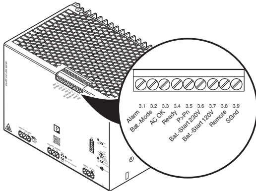
Figure 14 Connection terminal block signaling (3.1...3.9)
