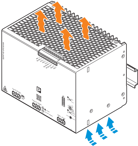
Figure 4 Convection
