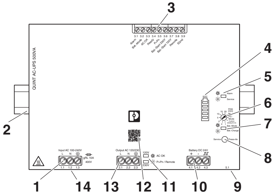
Figure 1 Position of the function elements
