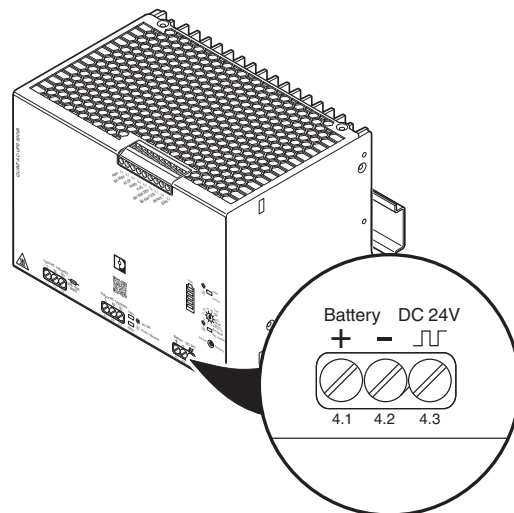
Figure 13 Battery connection terminal blocks: Battery DC +/-/Signal (4.1...4.3)
