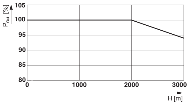
Figure 27 Altitude-dependent derating
