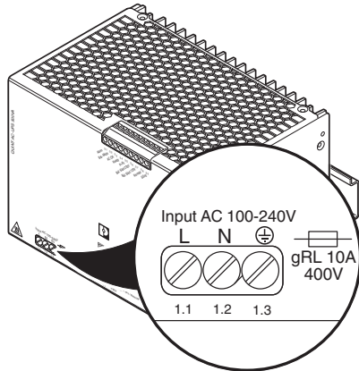
Figure 11 Input voltage connection terminal blocks: Input AC L/N/⊕ (1.1...1.3)
