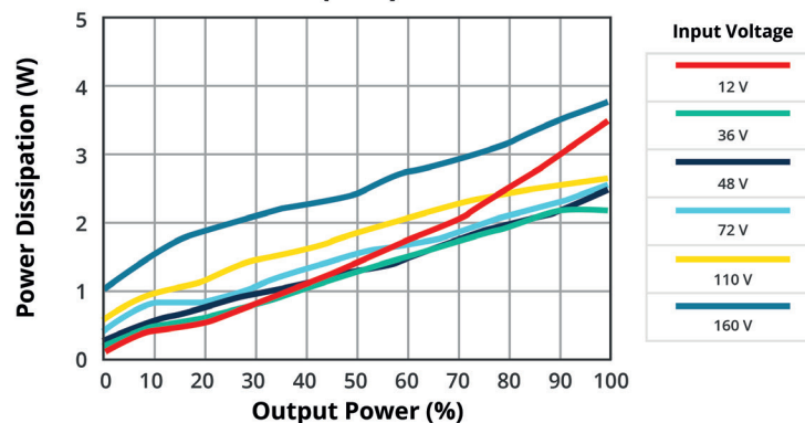
POWER DISSIPATION VS OUTPUT POWER PRFE20W-072-S12-D (25°C)
