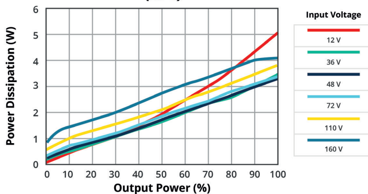
POWER DISSIPATION VS OUTPUT POWER PRFE20W-072-S5-D (25°C)
