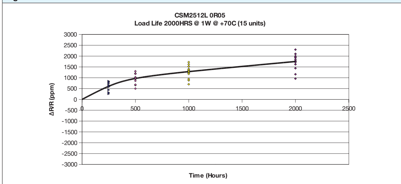
Figure 3 – Load Life Results of CSM2512L
