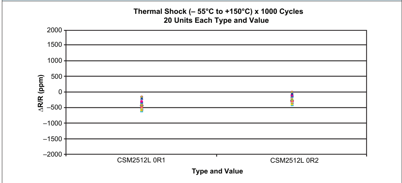
Figure 4 – Thermal Shock Results of CSM2512L
