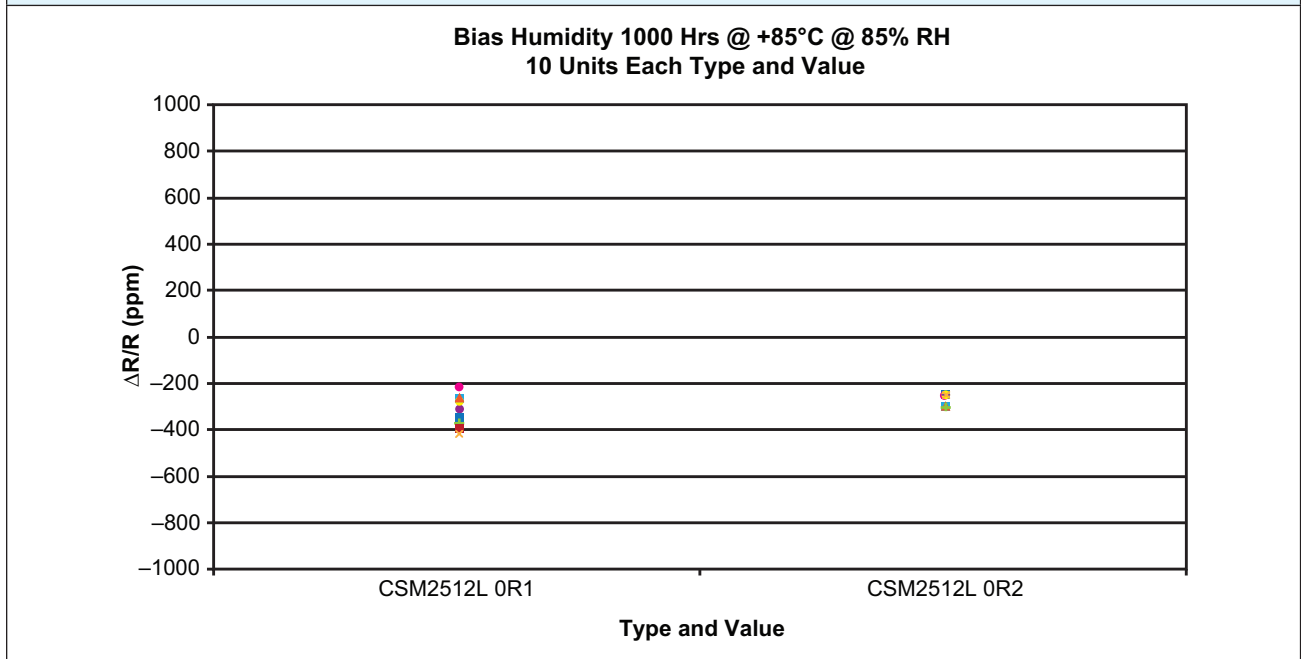
Figure 5 – Bias Humidity Results of CSM2512L
