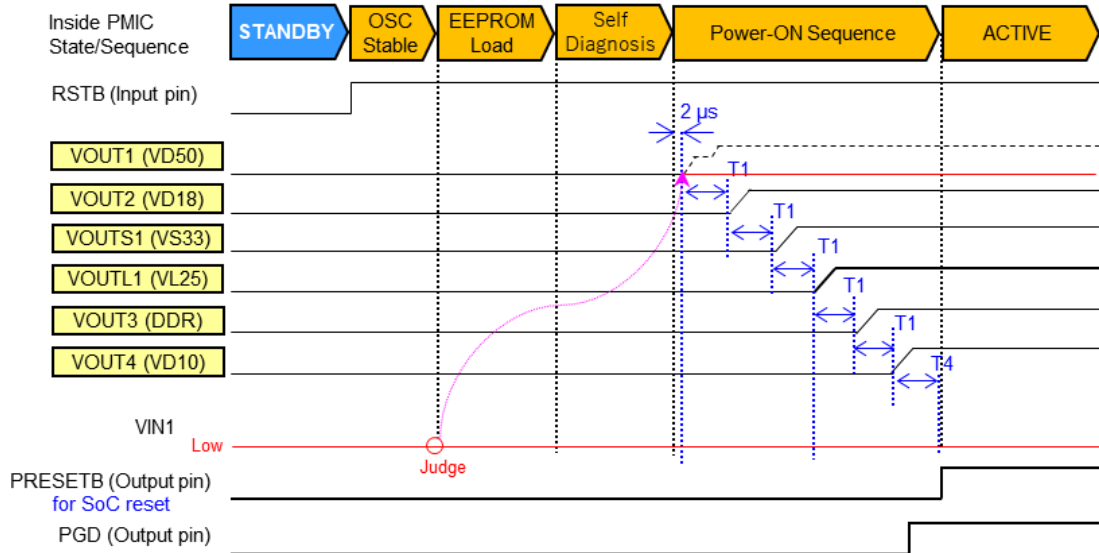
Figure 16. VOUT1 Disable Setting without EEPROM
