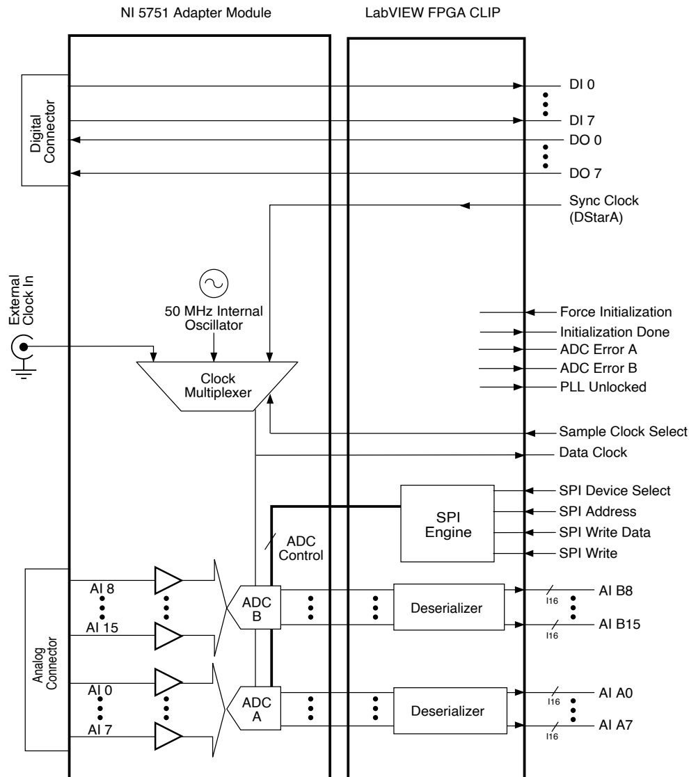
Figure 1. NI 5751 Hardware Block Diagram
