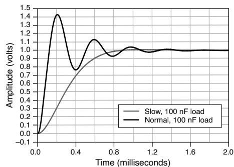
Figure 1. 1 mA Range, 100 nF Load Step Response, Typical
