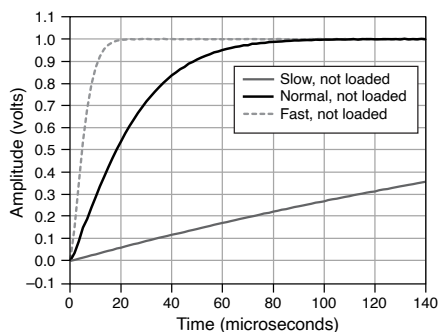
Figure 1. 1 mA Range No Load Step Response, Typical
