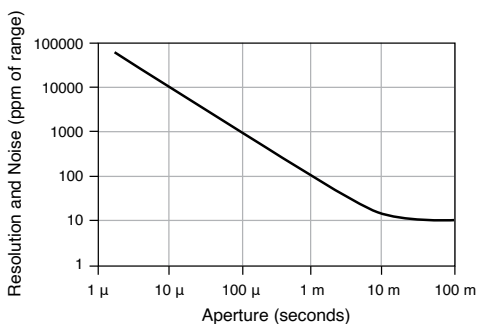
Figure 1. Noise and Resolution versus Measurement Aperture, Typical
