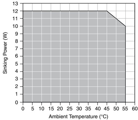
Figure 4. Sinking Power vs. Ambient Temperature Derating
