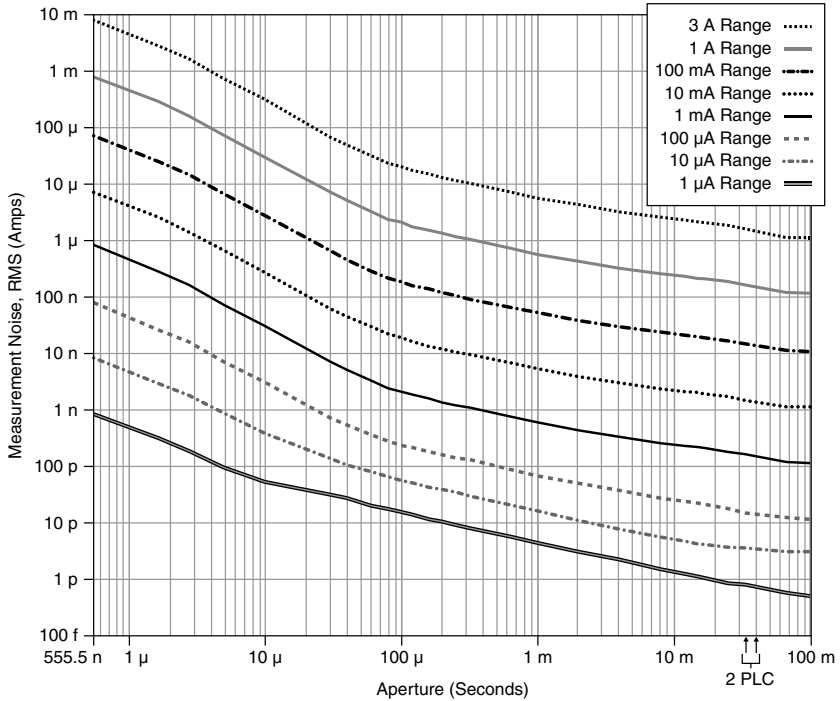
Figure 3. Current Measurement Noise vs. Measurement Aperture, Nominal
