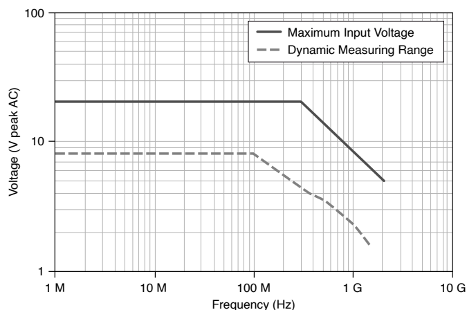
Figure 3. SA1500X Maximum Input Voltage Versus Frequency. Derate voltage according to the frequency of the signal you are measuring.
