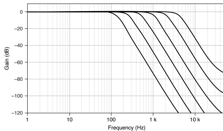
Figure 6. Butterworth Filter Magnitude Response (4th Order, with 12.8 MHz Timebase)
