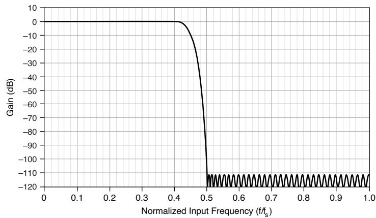
Figure 1. Brickwall Filter Magnitude Response
