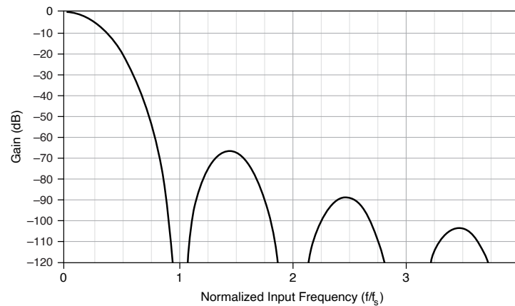
Figure 7. Comb Filter Magnitude Response
