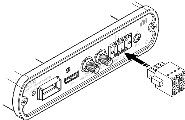
Figure 4. Connecting the 8-Pin Female Connector to the DIO Spring Terminals
