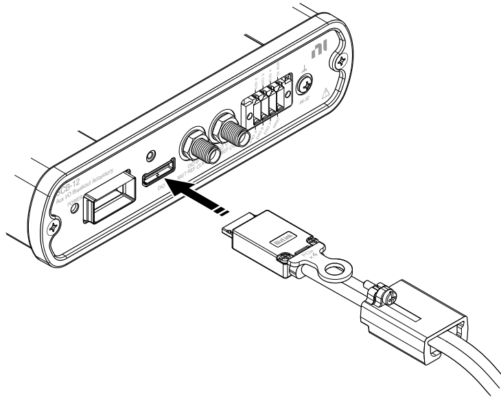
Figure 4. Connecting the Strain Relief Assembly
