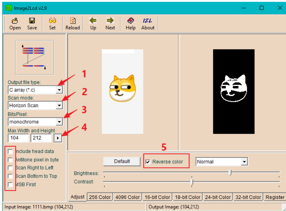
Figure 4. Image2LCD configuration
