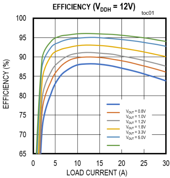
Efficiency curves
