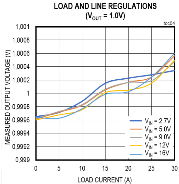
Load line regulation
