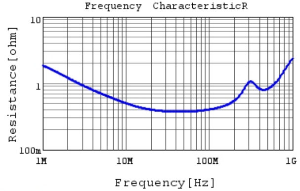
DE2E3SA332MN3AY02F R DC0V, 20degC
