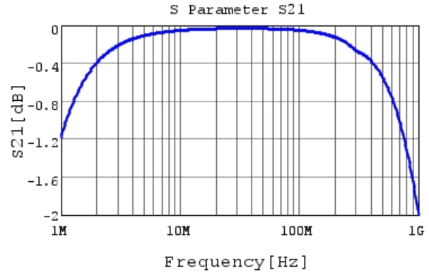
DE2E3SA332MN3AY02F S21 DCOV, 20degC
