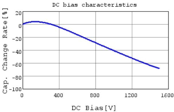
DE2E3SA332MN3AY02F C-DC bias capchange, 20.0
