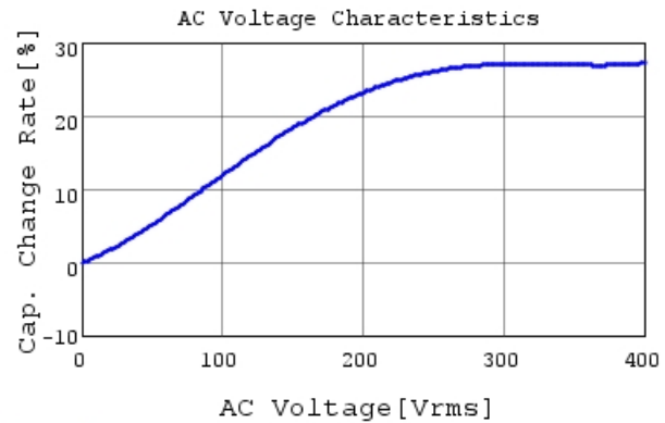
DE2E3SA332MN3AY02F C-AC Voltage capchange, I
