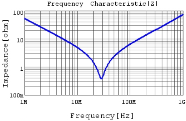
DE2E3SA332MN3AY02F |Z| DC0V, 20degC
