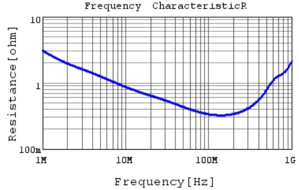
DE2E3SA152MN3AT02F R DCOV, 20degC
