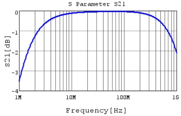
DE2E3SA152MN3AT02F S21 DCOV, 20degC
