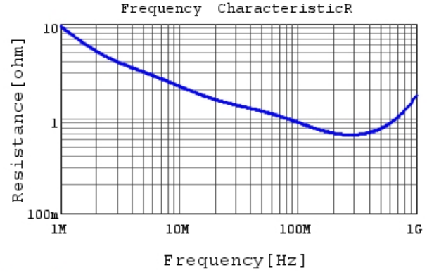
DE2B3SA471KA2BT01F R DC0V, 20degC
