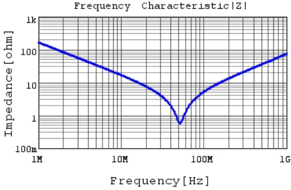
DE1E3RA102MN4AQ01F |Z| DCOV, 20degC
