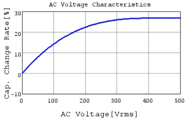
DE1E3RA102MN4AQ01F C-AC Voltage capchange, I
