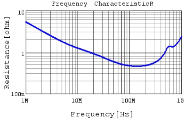
DE1E3RA102MN4AQ01F R DCOV, 20degC
