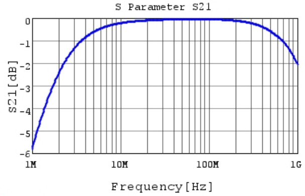
DE1E3RA102MN4AQ01F S21 DCOV, 20degC
