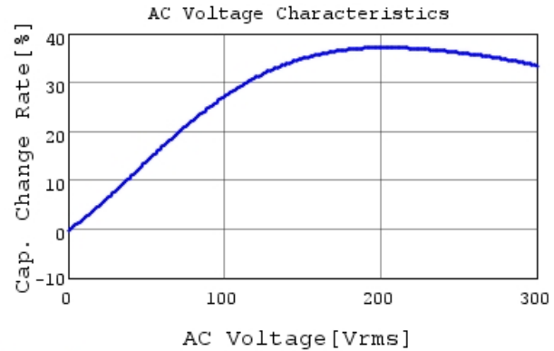
DE2E3SA102MN3AX02F C-AC Voltage capchange, I
