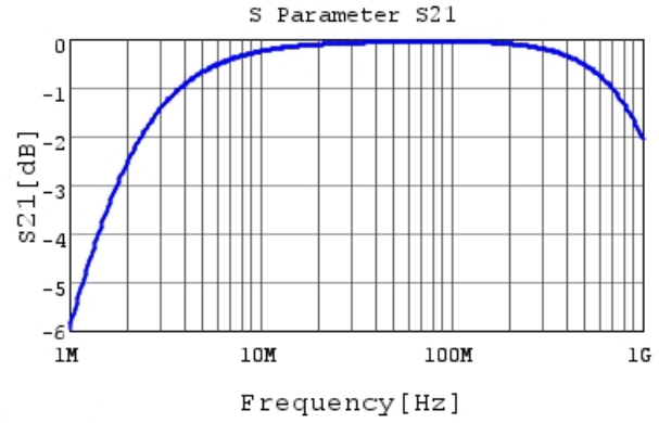
DE2E3SA102MN3AX02F S21 DCOV, 20degC
