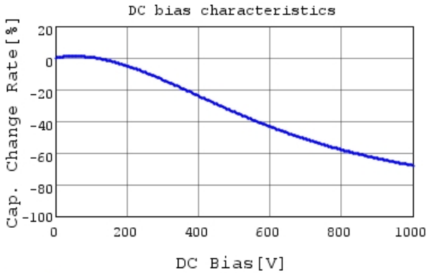
DE2E3SA102MN3AX02F C-DC bias capchange, 20.0
