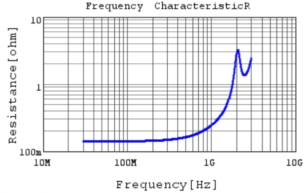
RCE5C3A680J2M1H03A R DC0V, 25degC
