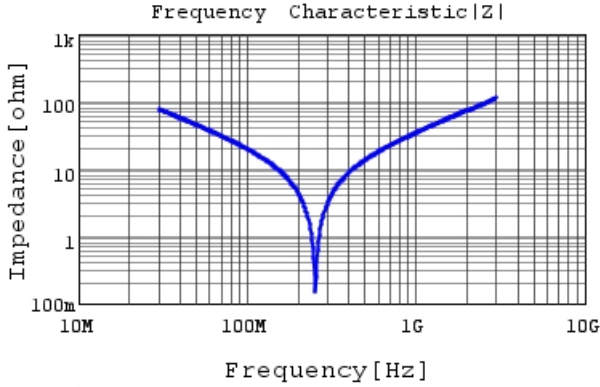
RCE5C3A680J2M1H03A |Z| DC0V, 25degC
