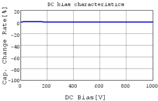
RCE5C3A680J2M1H03A C-DC bias capchange, 25.0
