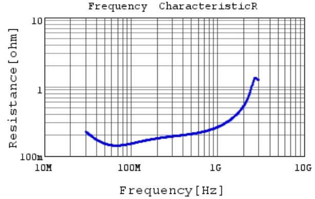
RCE5C2J560J1K1H03B R DC0V, 25degC
