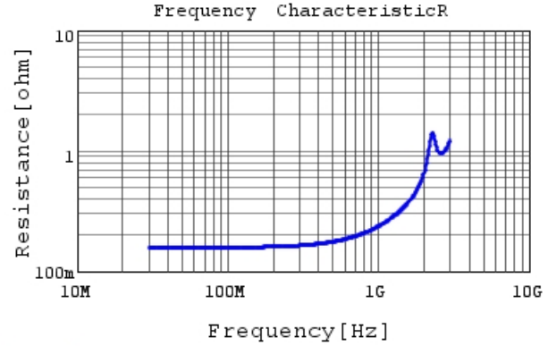
RCE5C2J680J1K1H03B R DC0V, 25degC
