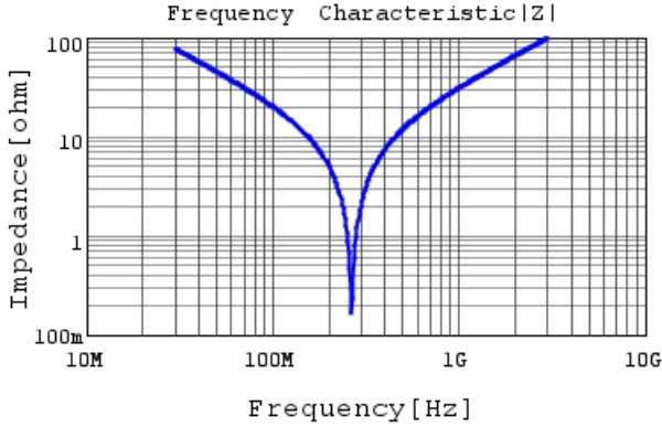
RCE5C2J680J1K1H03B |Z| DC0V, 25degC
