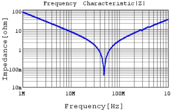
RCE5C2J222J1K1H03B |Z| DC0V, 25degC
