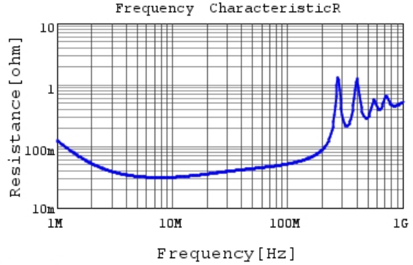
RCE5C2J222J1K1H03B R DC0V, 25degC
