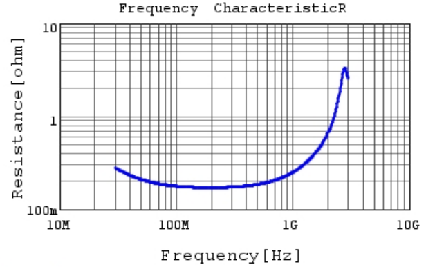
RDE5C3A470J2K1H03B R DC0V, 25degC
