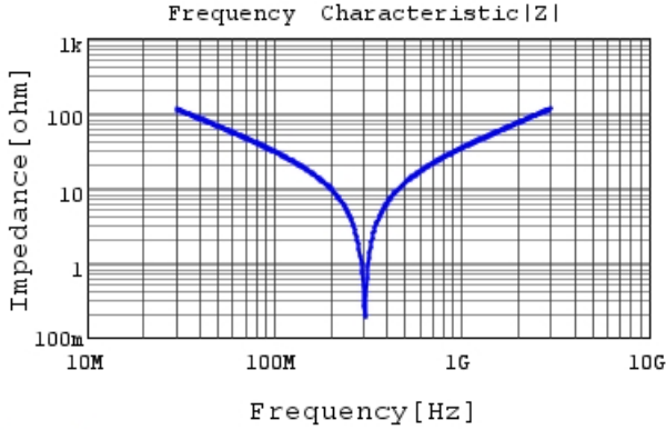
RDE5C3A470J2K1H03B |Z| DC0V, 25degC
