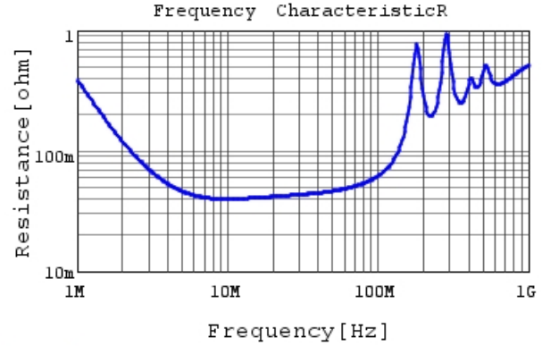
RDE5C2J392J2K1H03B R DC0V, 25degC
