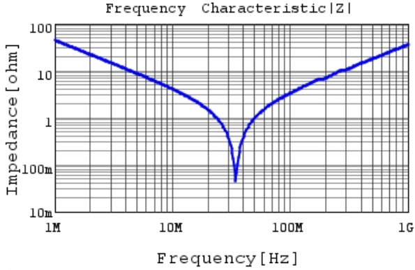
RDE5C2J392J2K1H03B |Z| DC0V, 25degC
