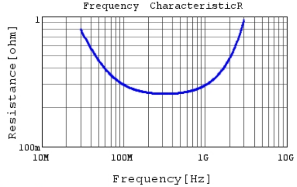
RDE5C2J220J1K1H03B R DC0V, 25degC
