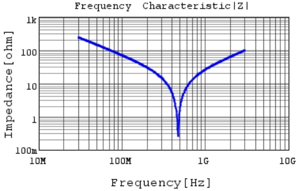
RDE5C2J220J1K1H03B |Z| DC0V, 25degC
