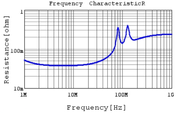
RDE5C2E183J2K1H03B R DC0V, 25degC
