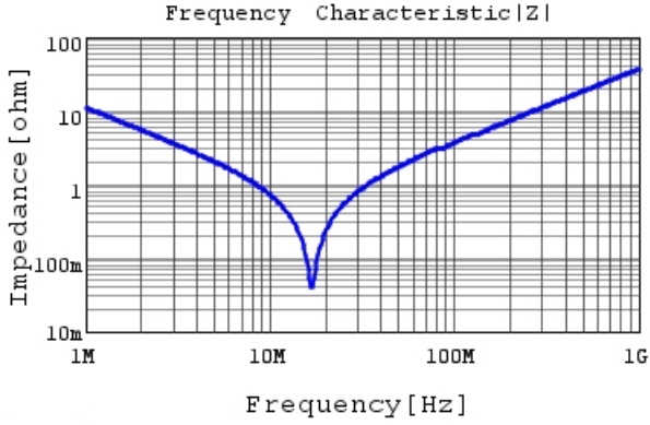
RDE5C2E183J2K1H03B |Z| DC0V, 25degC
