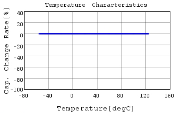
RDE5C2E183J2K1H03B C-Temp. capchange, DC0V,
