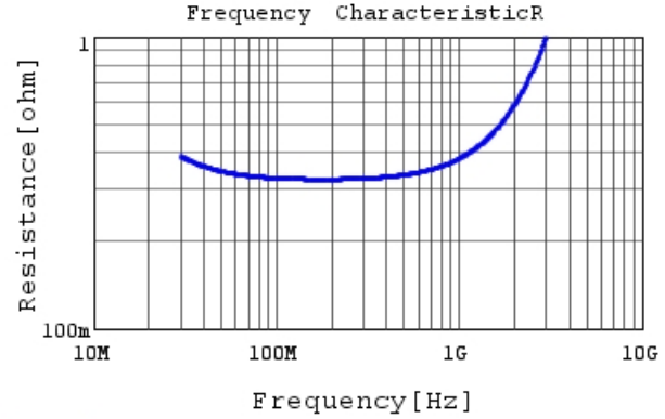
RDE5C2J120J1K1H03B R DC0V, 25degC
