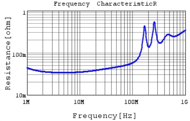
RDE5C2E682J1K1H03B R DC0V, 25degC
