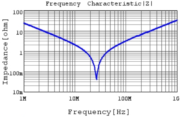
RDE5C2E682J1K1H03B |Z| DC0V, 25degC
