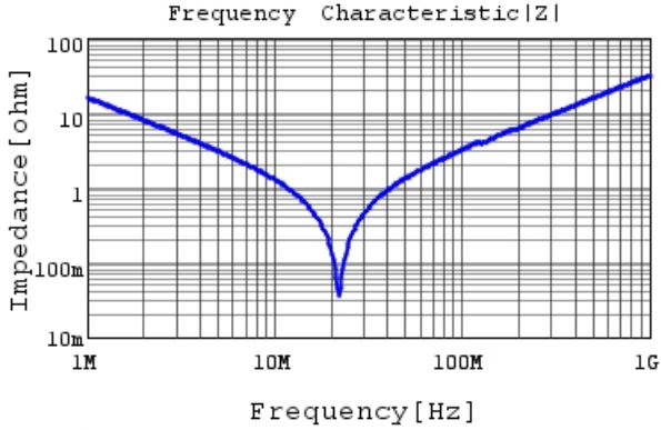
RCE5C2E103J1K1H03B |Z| DC0V, 25degC
