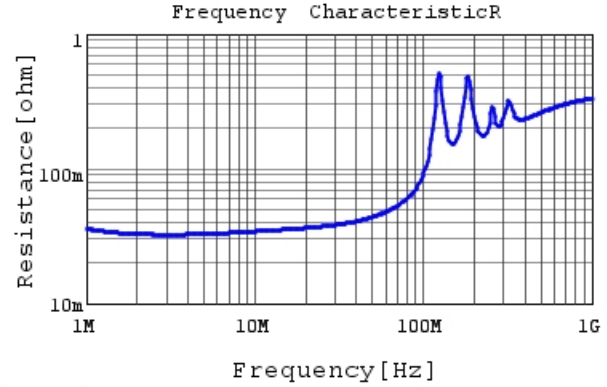
RCE5C2E103J1K1H03B R DC0V, 25degC
