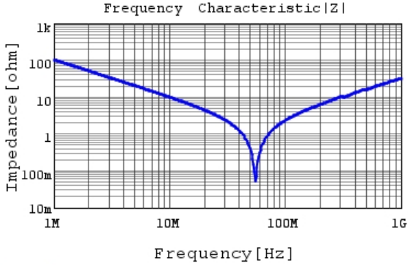
RCE5C2J182J1K1H03B |Z| DC0V, 25degC
