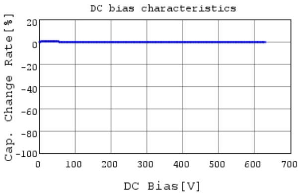
RCE5C2J182J1K1H03B C-DC bias capchange, 25.0
