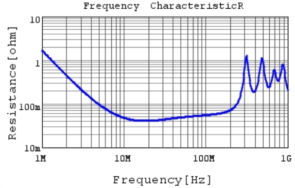
RCE5C2J182J1K1H03B R DC0V, 25degC
