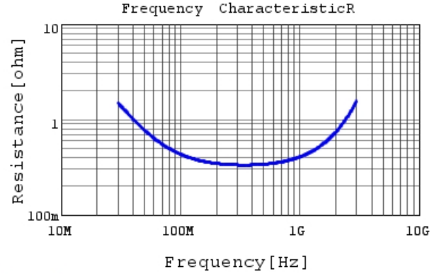
RCE5C3A150J2K1H03B R DC0V, 25degC
