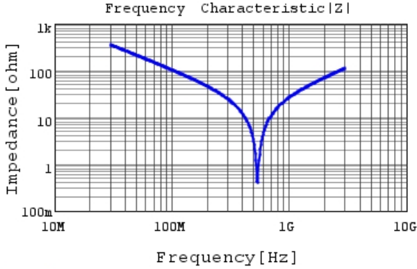
RCE5C3A150J2K1H03B |Z| DC0V, 25degC
