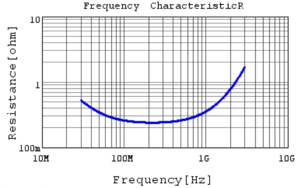
RDE5C2J270J1K1H03B R DC0V, 25degC
