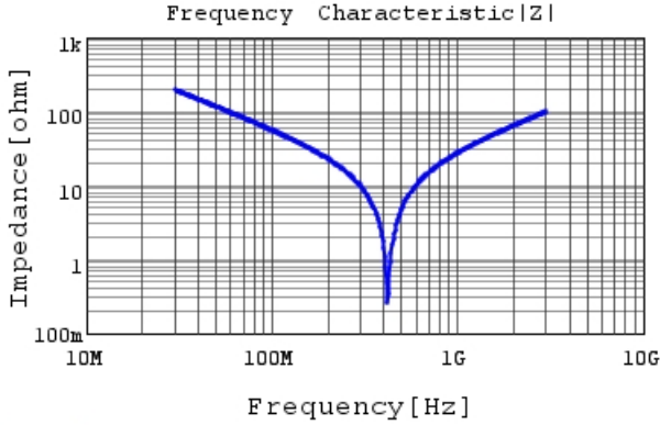
RDE5C2J270J1K1H03B |Z| DC0V, 25degC
