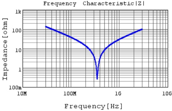
RDE5C2J390J1K1H03B |Z| DC0V, 25degC
