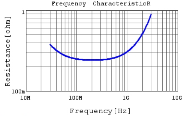
RDE5C2J390J1K1H03B R DC0V, 25degC
