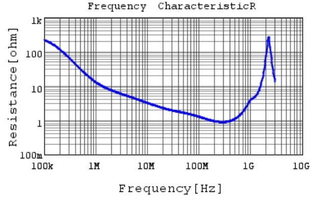
DE6B3KJ331KA3BE01J R DC0V, 20degC
