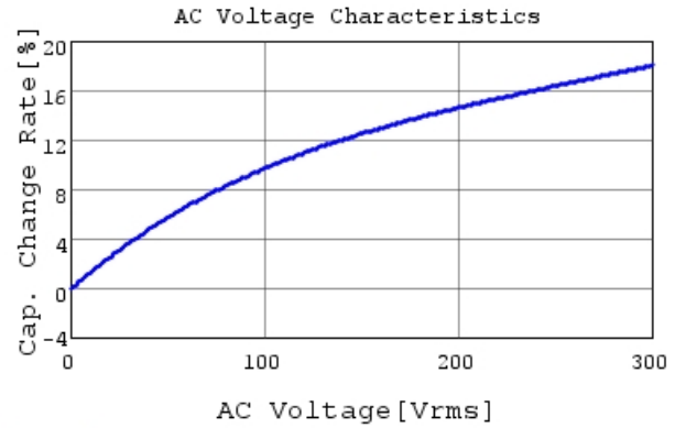
DE6B3KJ331KA3BE01J C-AC Voltage capchange, I
