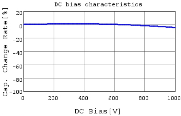
DE6B3KJ331KA3BE01J C-DC bias capchange, 20.0
