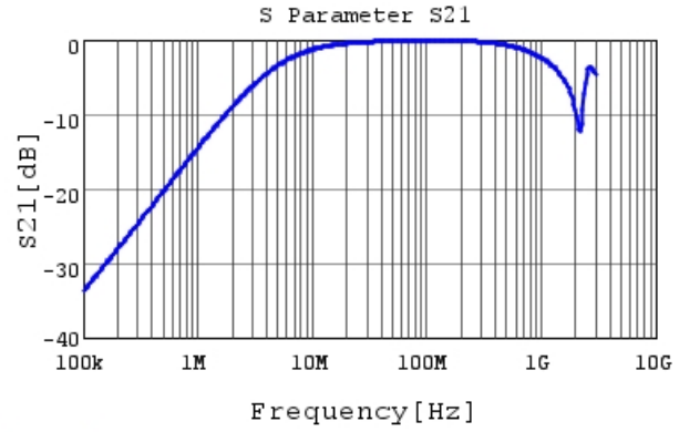
DE6B3KJ331KA3BE01J S21 DCOV, 20degC
