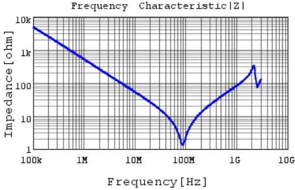
DE6B3KJ331KA3BE01J |Z| DC0V, 20degC
