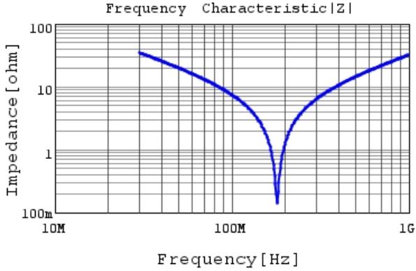
RCE5C2J151J1K1H03B |Z| DC0V, 25degC
