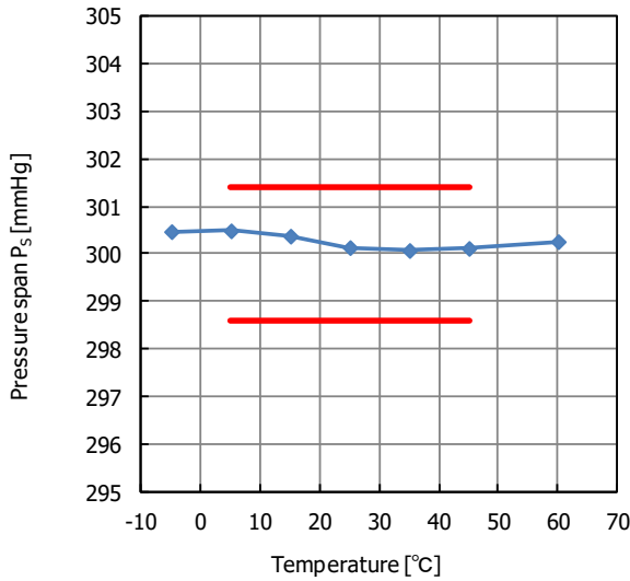
Fig.20.13 Pressure span P s temperature characteristic (note 9 )
