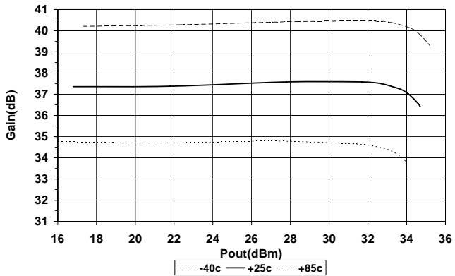
Typical Gain vs Pout, F=2.4GHz
