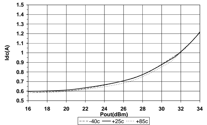
DC Supply Current vs Pout, F=2.7GHz
