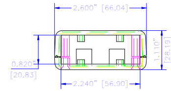
ASSEMBLED VIEW
