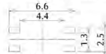
Reference land dimension
