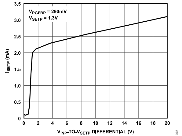
Figure 75. I_{SETP} during Start-Up with Fast Start-Up Enabled vs. V_{INP} -to- V_{SETP} Differential
