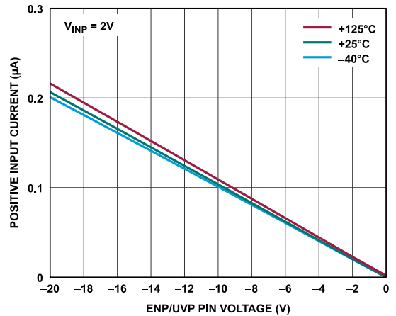
Figure 51. Positive Input Current vs. ENP/UVP Pin Voltage
