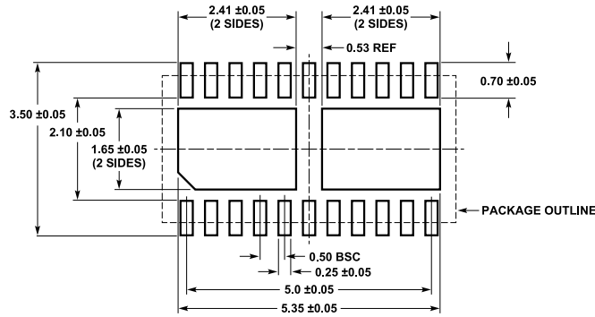
RECOMMENDED SOLDER PAD PITCH AND DIMENSIONS APPLY SOLDER MASK TO AREAS THAT ARE NOT SOLDERED
