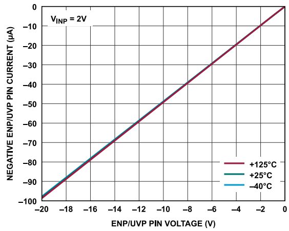
Figure 50. Negative ENP/UVP Pin Current vs. ENP/UVP Pin Voltage
