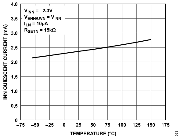
Figure 23. INN Quiescent Current vs. Temperature ( V_{ENN/UVN} = V_{INN} )
