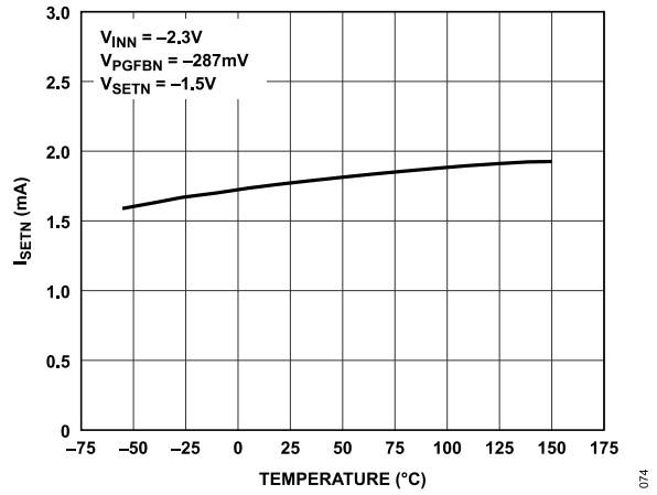
Figure 74. I_{SETN} during Start-Up with Fast Start-Up Enabled vs. Temperature
