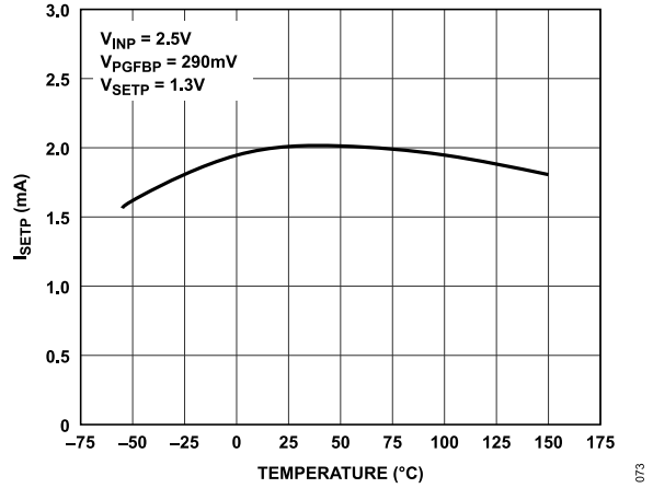
Figure 73. I_{SETP} during Start-Up with Fast Start-Up Enabled vs. Temperature
