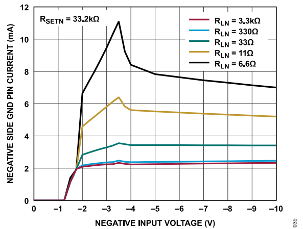
Figure 39. Negative Side GND Pin Current vs. Negative Input Voltage ( R_{LN} is the Negative Load Resistance)
