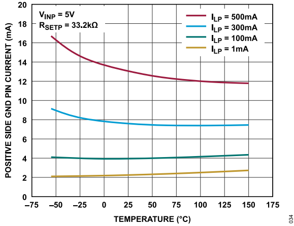
Figure 34. Positive Side GND Pin Current vs. Temperature
