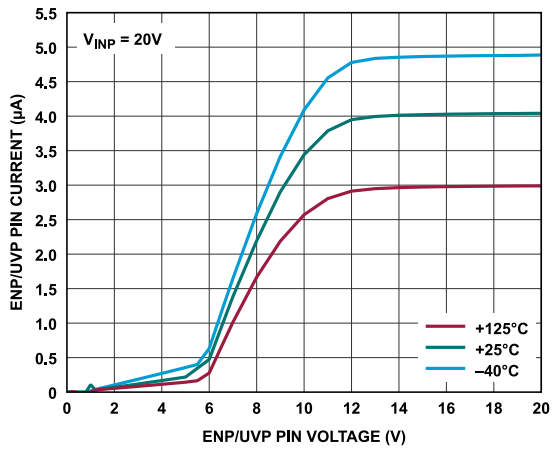
Figure 47. ENP/UVP Pin Current vs. ENP/UVP Pin Voltage (Temperature Steps)
