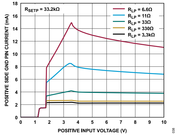
Figure 38. Positive Side GND Pin Current vs. Positive Input Voltage ( R_{LP} is the Positive Load Resistance)
