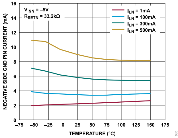
Figure 35. Negative Side GND Pin Current vs. Temperature
