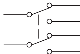
CIRCUIT DIAGRAM (DPDT) ON-ON
